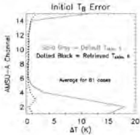
Figure 2: Initial brightness temperature error in two retrieval approaches implemented using the NRL 1DVAR routine. The gray line corresponds to retrievals which used NOGAPS land surface temperature and a fixed emissivity of 0.9; while the dotted black line corresponds to retrievals which included the CIRA retrieved GOES land surface temperature and AMSU-A emissivities.
