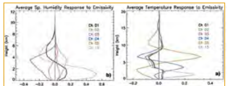
Figure 4: Response of atmospheric temperature and specific humidity profiles to perturbations in emissivity for AMSU-A channels. Shown are responses of a) temperature to emissivity, and b) specific humidity to emissivity.
