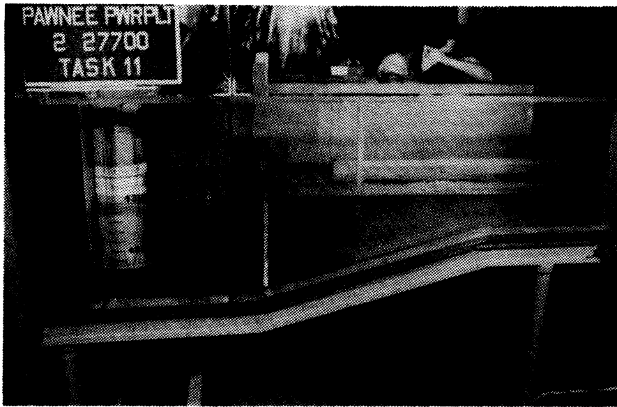
Figure 8. Pump Operation in a Modified Sump with Baffle Plates, Curtain Walls and Divider Wall in Place
